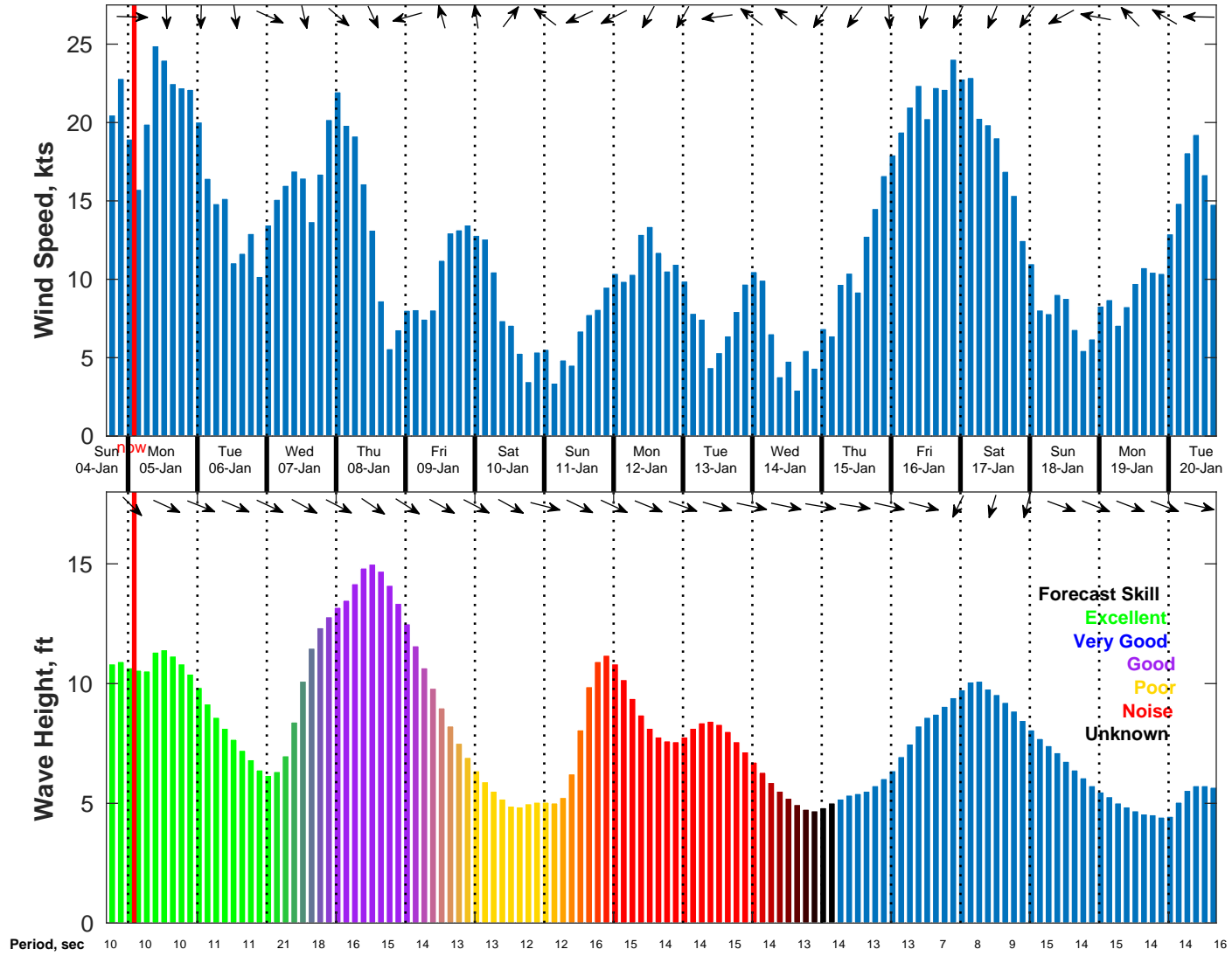
Wind & Wave Forecast for NDBC 46059 from 04-Jan-2026 17:00:00 to 20-Jan-2026 17:00:00
