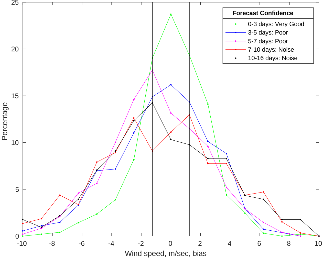
NDBC 46069 vs GFS Winds Bias Histogram: 05-Jan-2026
