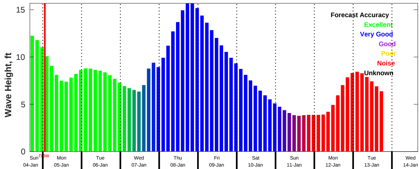
CMEMS Wave Forecast for NDBC 46259 from 04-Jan-2026 16:00:00 to 14-Jan-2026 16:00:00
