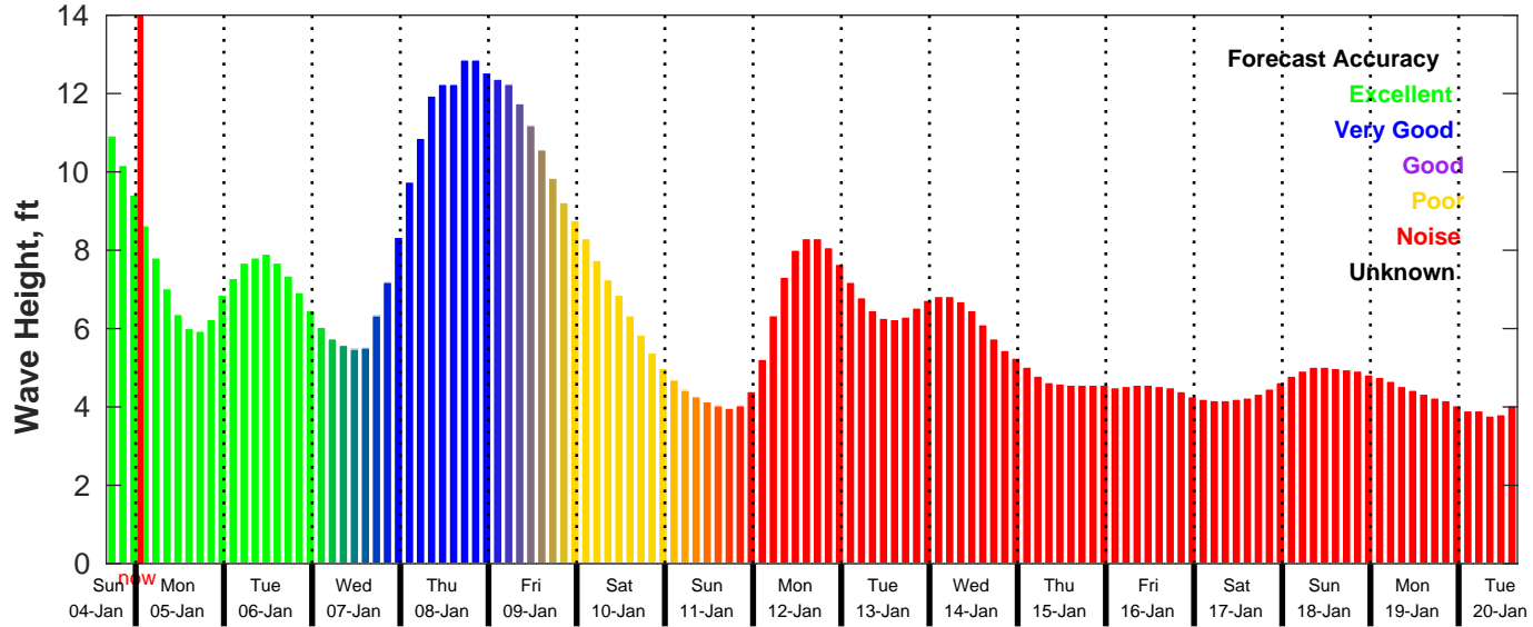
GFS Wave Forecast for NDBC 46259 from 04-Jan-2026 16:00:00 to 20-Jan-2026 16:00:00
