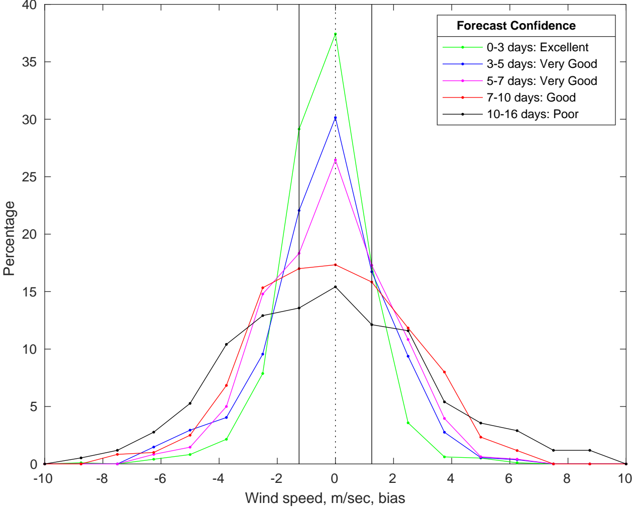
NDBC 51000 vs GFS Winds Bias Histogram: 05-Jan-2026
