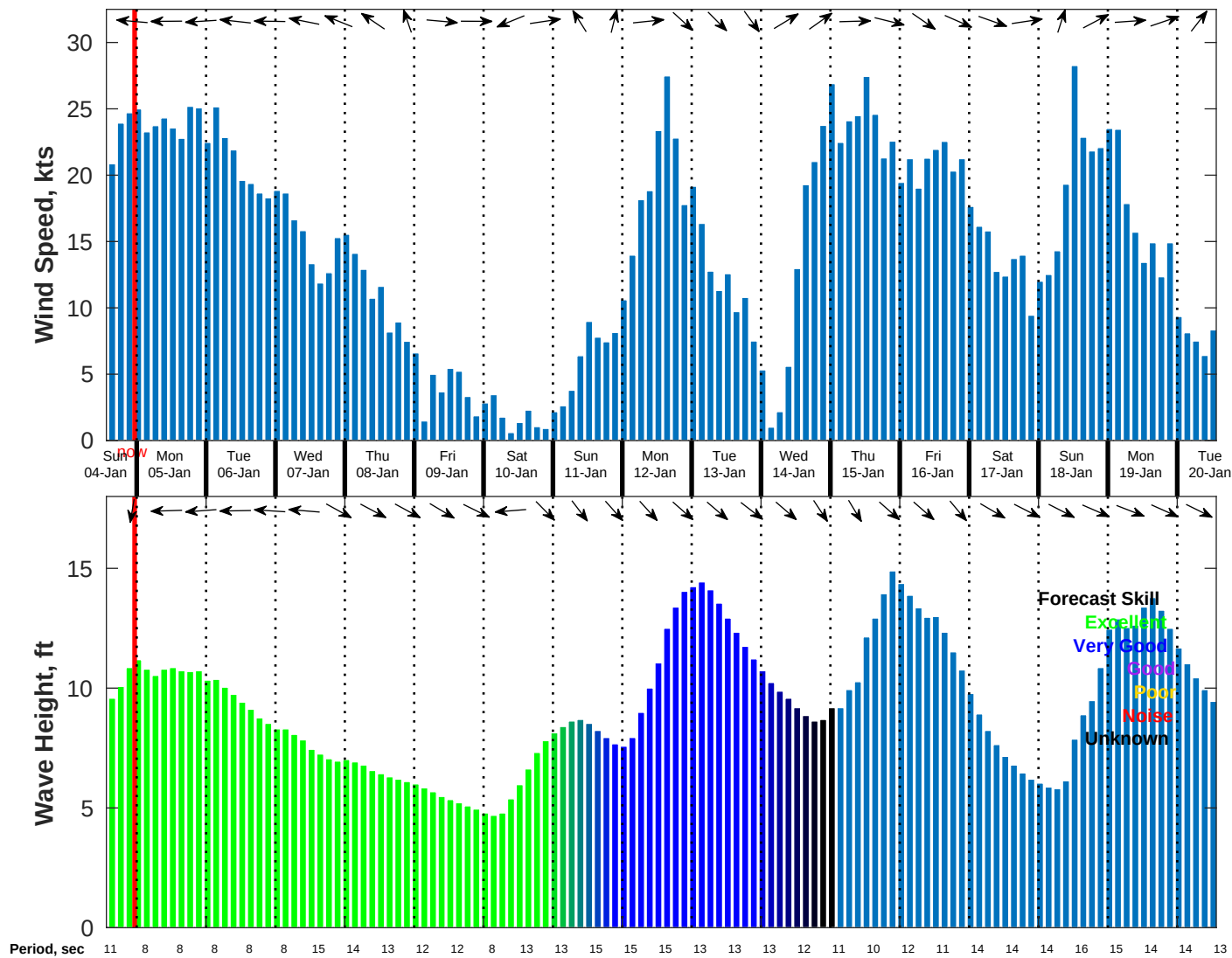
Wind & Wave Forecast for NDBC 51000 from 04-Jan-2026 14:00:00 to 20-Jan-2026 14:00:00
