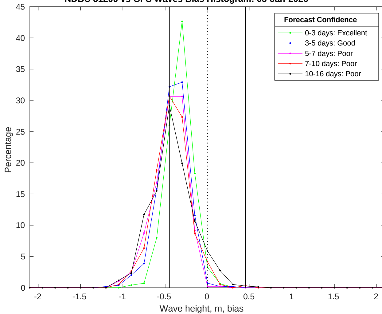
NDBC 51209 vs GFS Waves Bias Histogram: 05-Jan-2026
