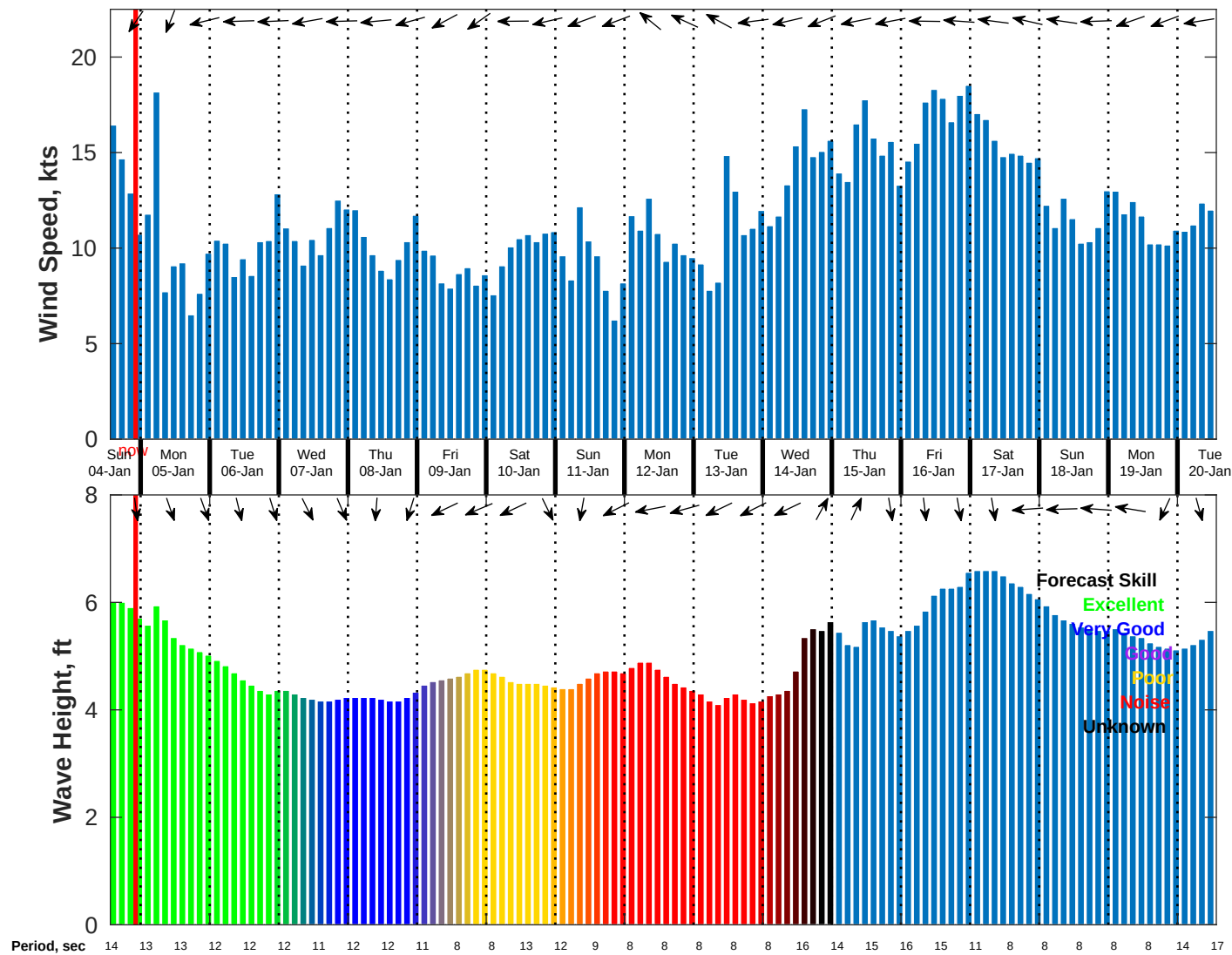
Wind & Wave Forecast for NDBC 51209 from 04-Jan-2026 13:00:00 to 20-Jan-2026 13:00:00
