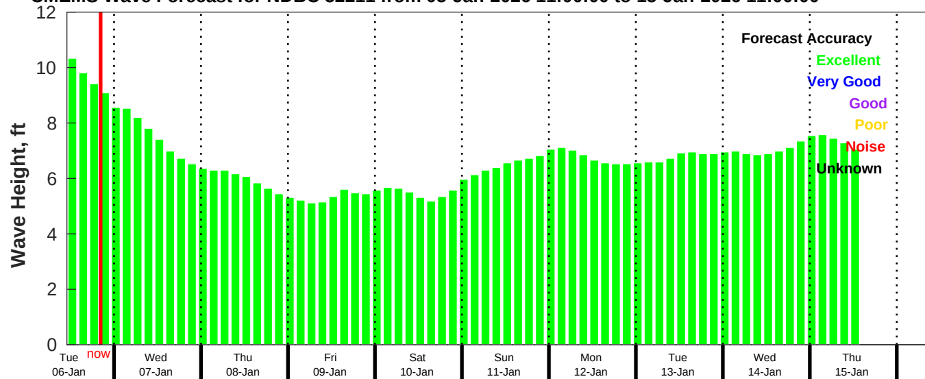
CMEMS Wave Forecast for NDBC 52211 from 05-Jan-2026 11:00:00 to 15-Jan-2026 11:00:00
