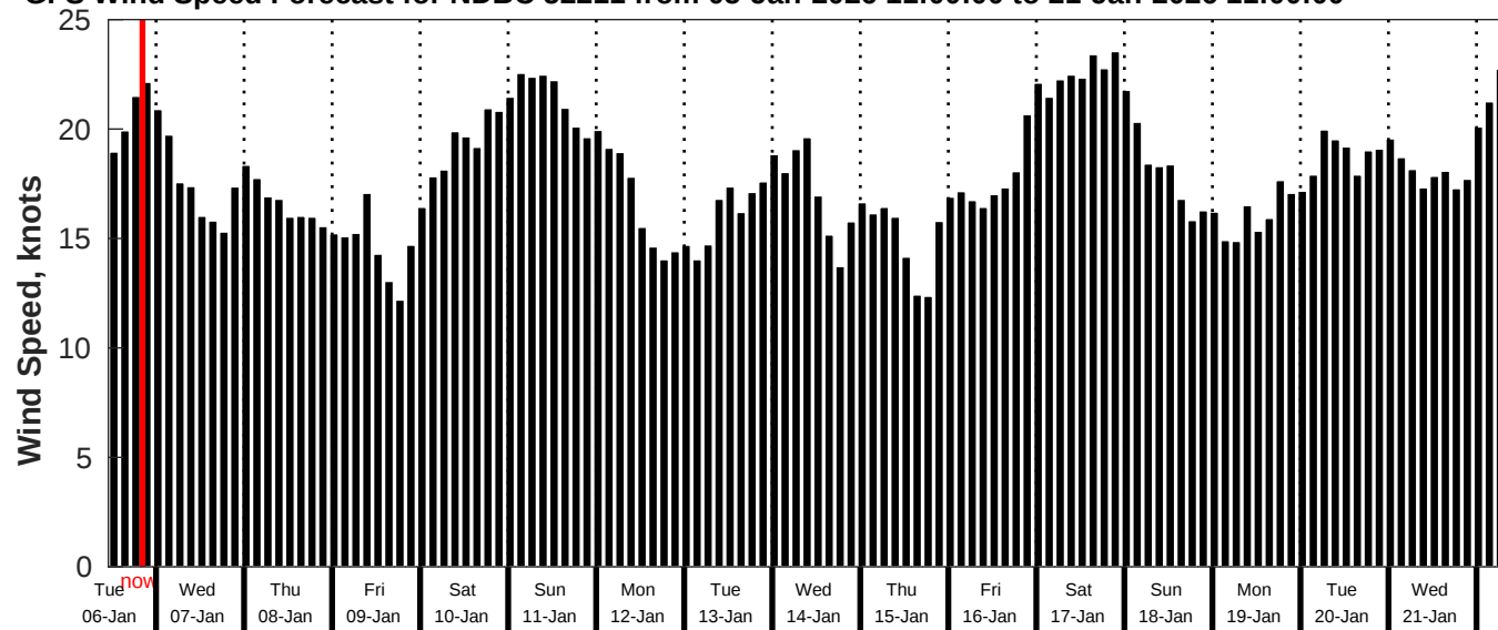
GFS Wind Speed Forecast for NDBC 52211 from 05-Jan-2026 11:00:00 to 21-Jan-2026 11:00:00
