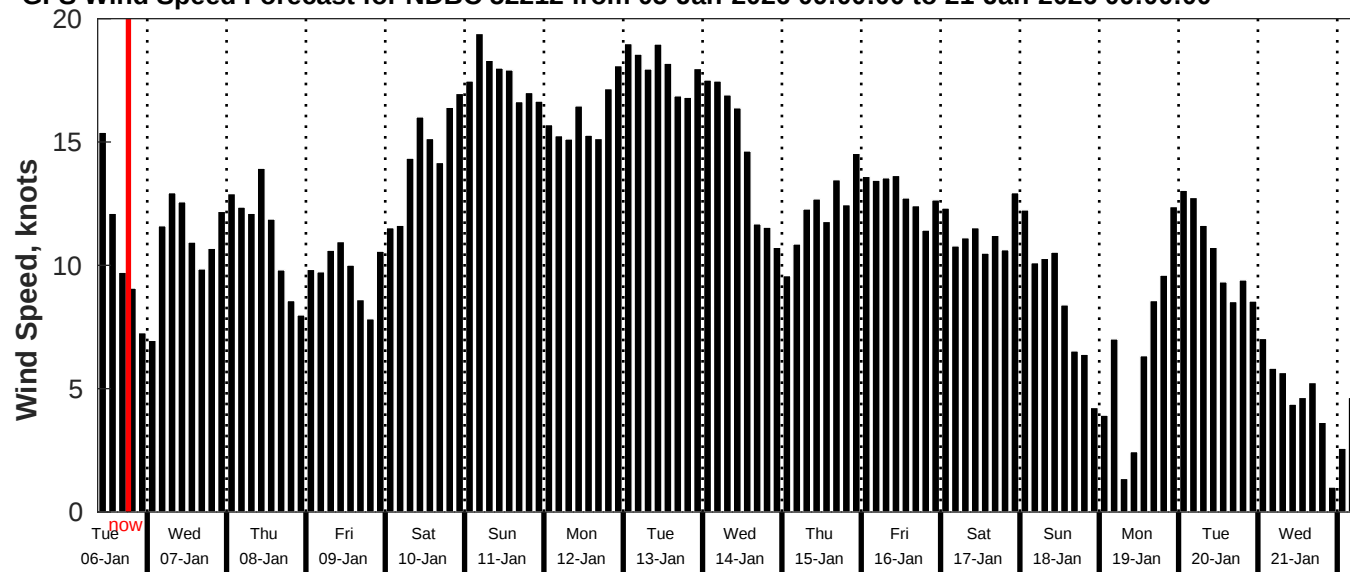
GFS Wind Speed Forecast for NDBC 52212 from 05-Jan-2026 09:00:00 to 21-Jan-2026 09:00:00
