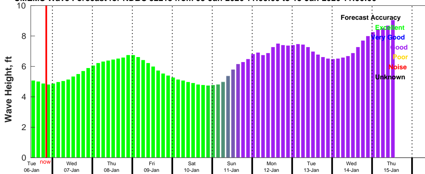
CMEMS Wave Forecast for NDBC 52213 from 05-Jan-2026 11:00:00 to 15-Jan-2026 11:00:00
