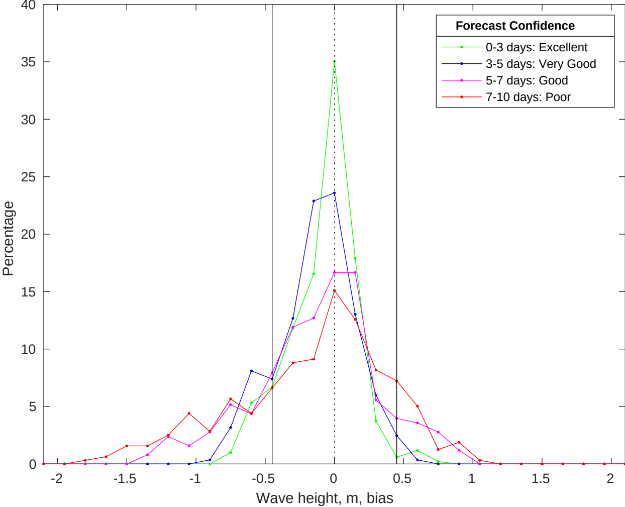
NDBC 41004 vs CMEMS Waves Bias Histogram: 06-Jan-2026
