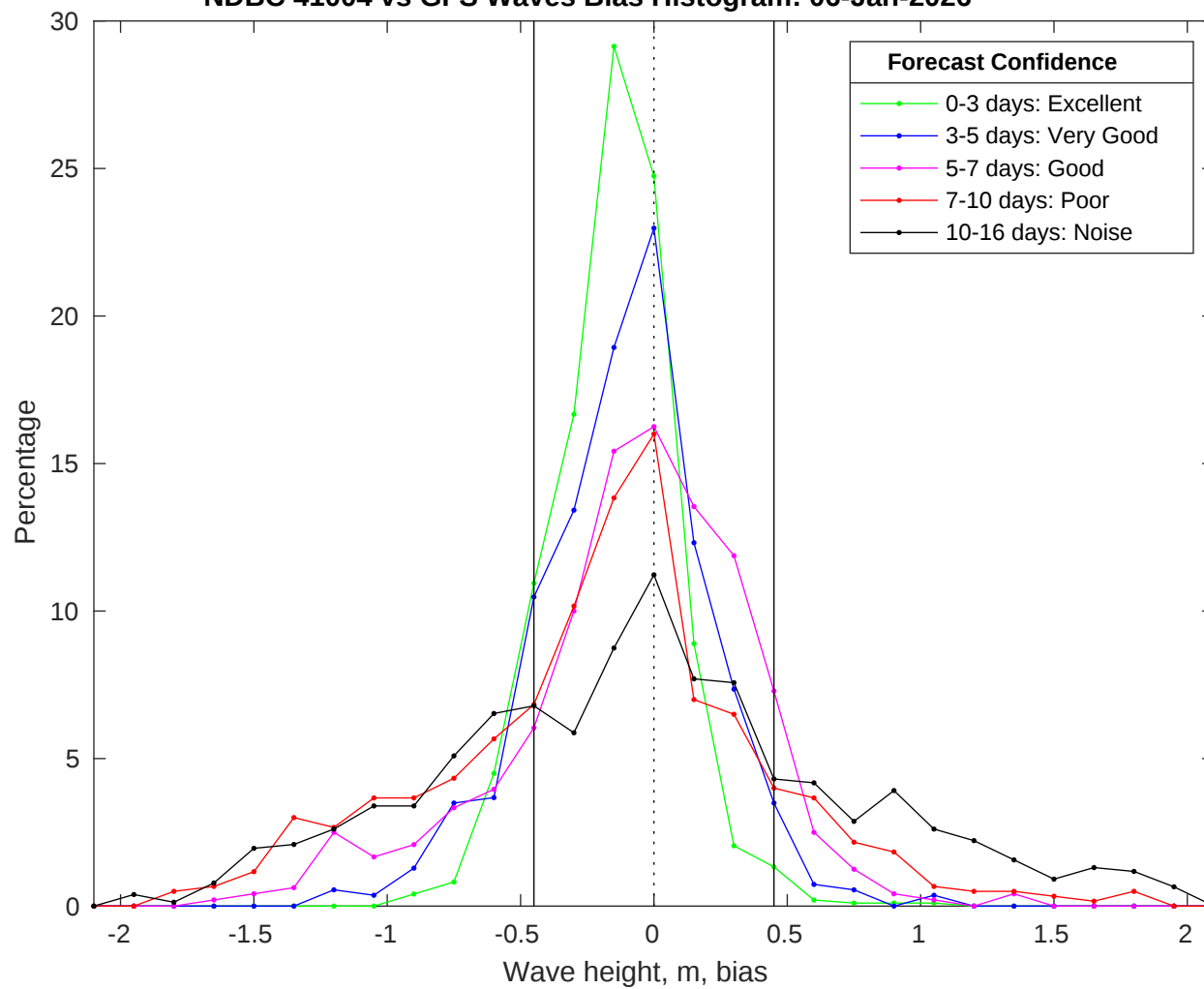
NDBC 41004 vs GFS Waves Bias Histogram: 06-Jan-2026
