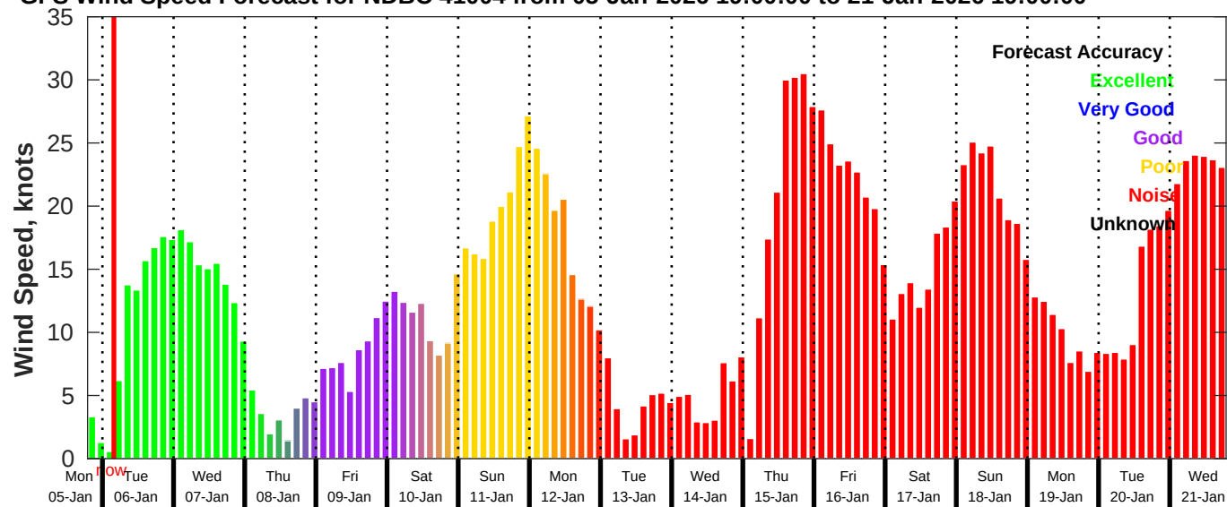
GFS Wind Speed Forecast for NDBC 41004 from 05-Jan-2026 19:00:00 to 21-Jan-2026 19:00:00
