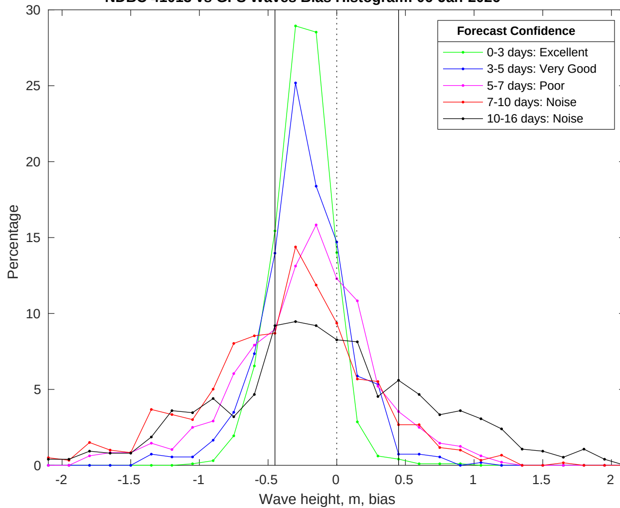
NDBC 41013 vs GFS Waves Bias Histogram: 06-Jan-2026
