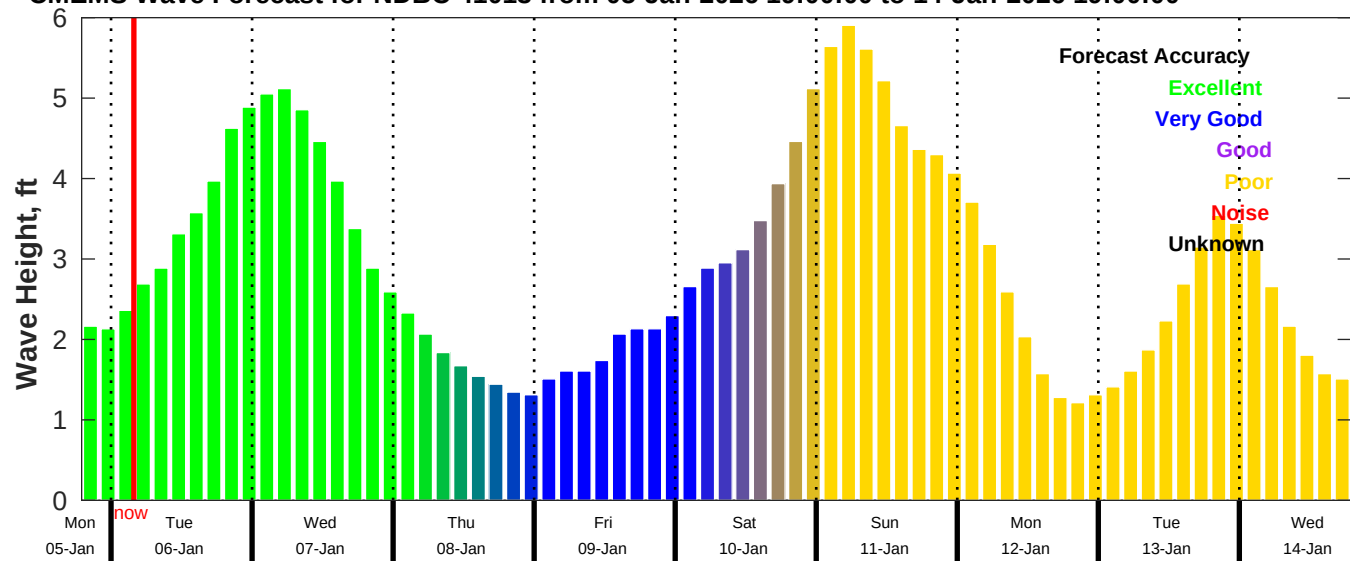
CMEMS Wave Forecast for NDBC 41013 from 05-Jan-2026 19:00:00 to 14-Jan-2026 19:00:00
