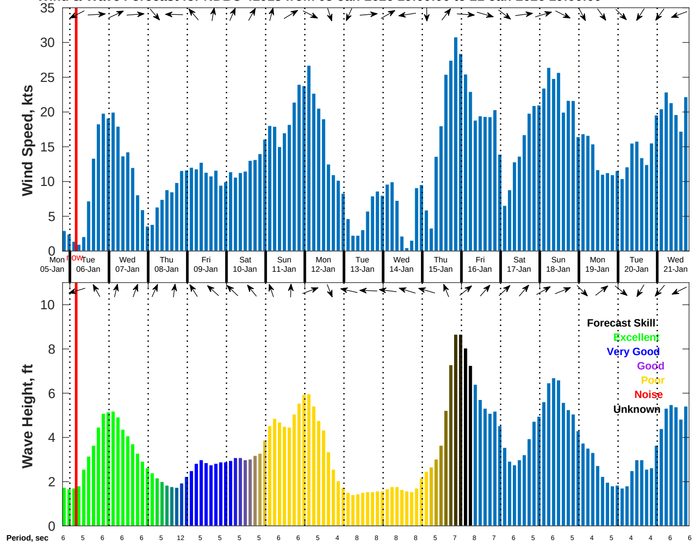
Wind & Wave Forecast for NDBC 41013 from 05-Jan-2026 19:00:00 to 21-Jan-2026 19:00:00
