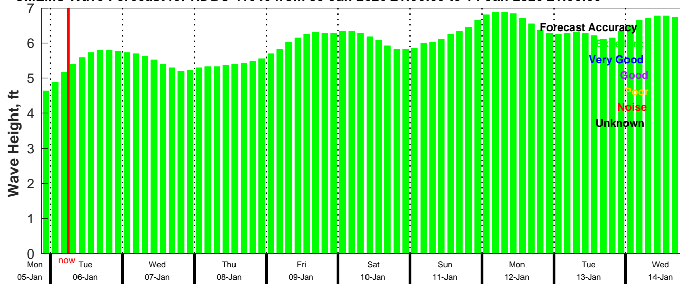
CMEMS Wave Forecast for NDBC 41040 from 05-Jan-2026 21:00:00 to 14-Jan-2026 21:00:00
