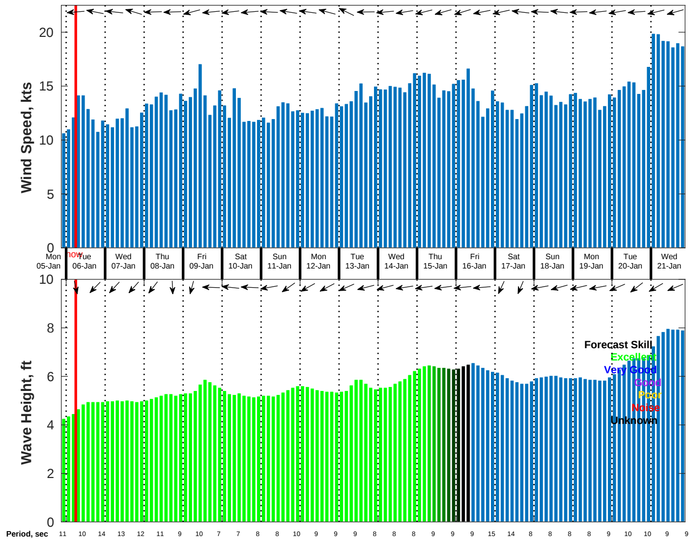
Wind & Wave Forecast for NDBC 41040 from 05-Jan-2026 21:00:00 to 21-Jan-2026 21:00:00
