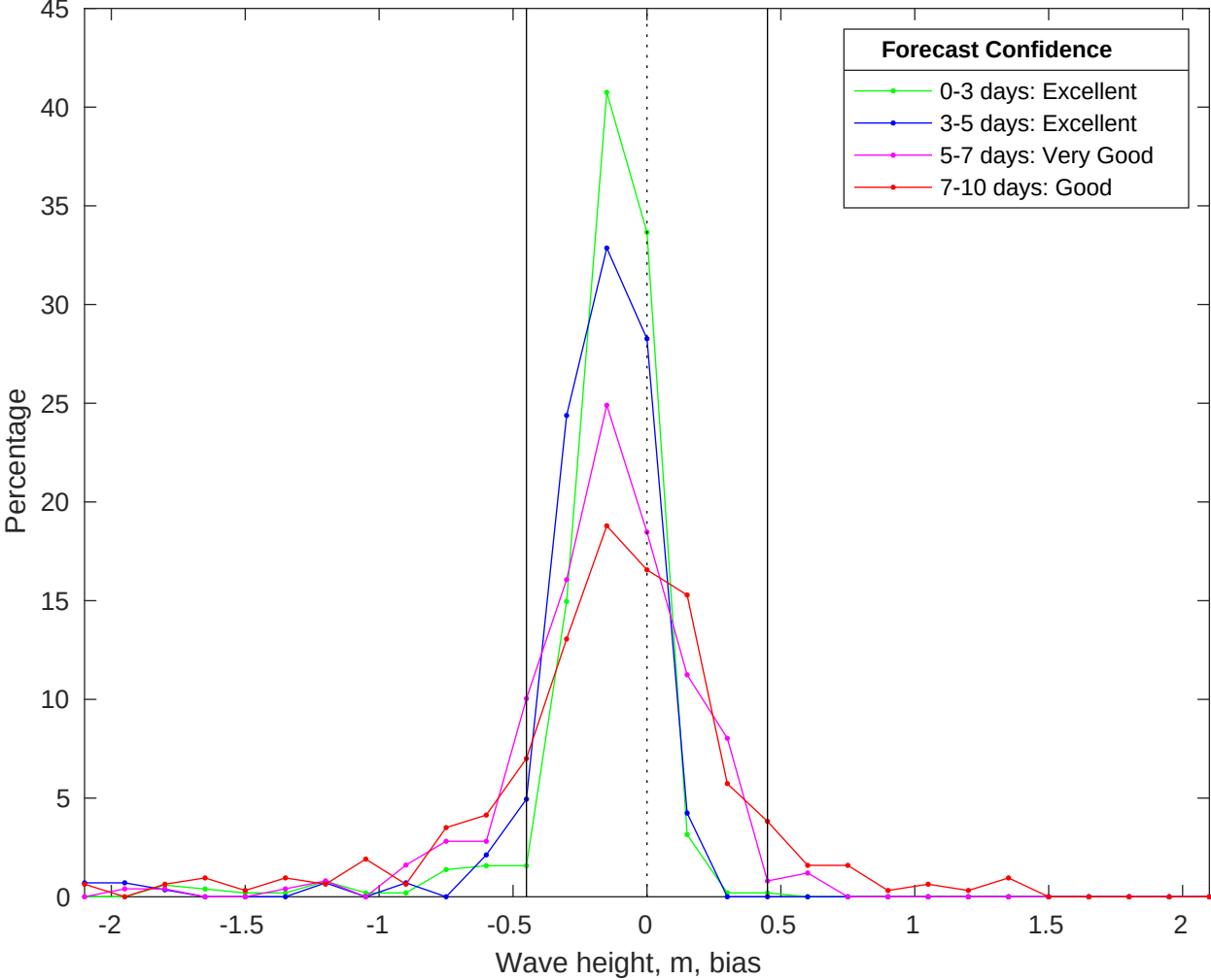
NDBC 42019 vs CMEMS Waves Bias Histogram: 06-Jan-2026
