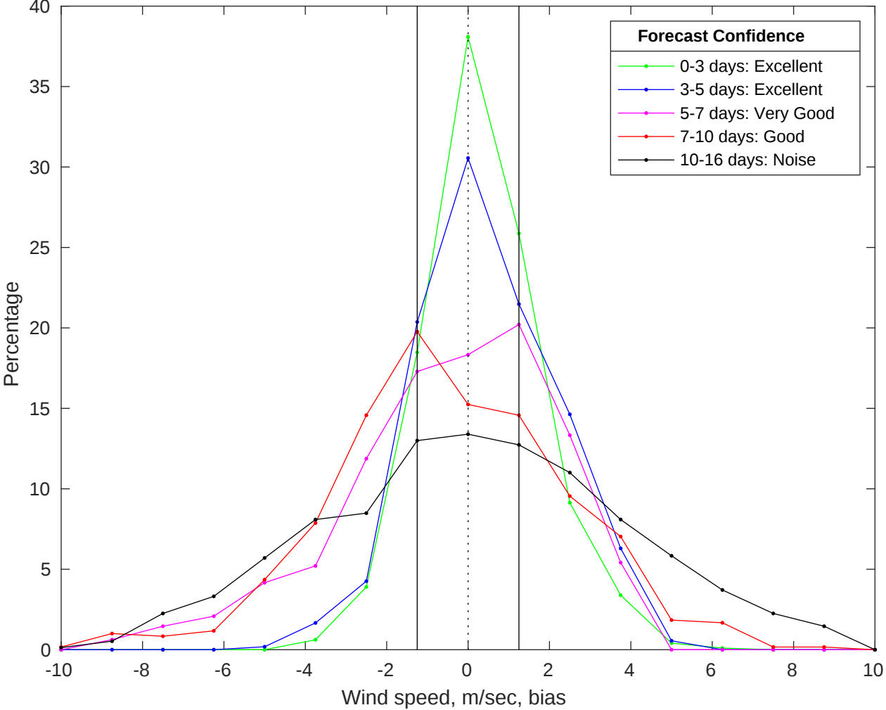
NDBC 42019 vs GFS Winds Bias Histogram: 06-Jan-2026
