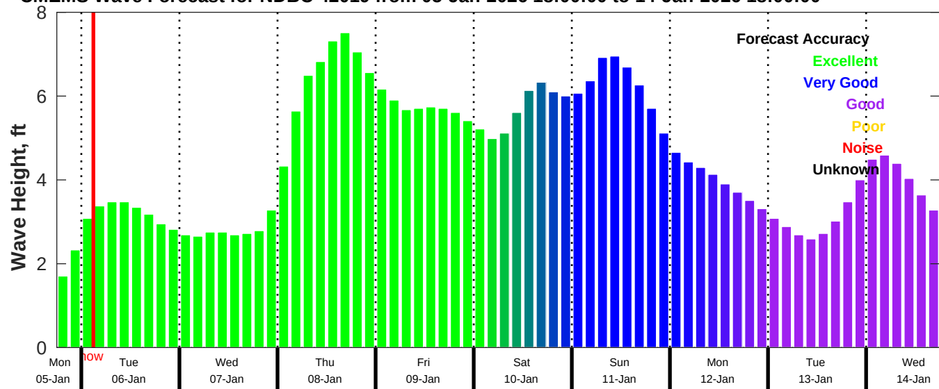
CMEMS Wave Forecast for NDBC 42019 from 05-Jan-2026 18:00:00 to 14-Jan-2026 18:00:00
