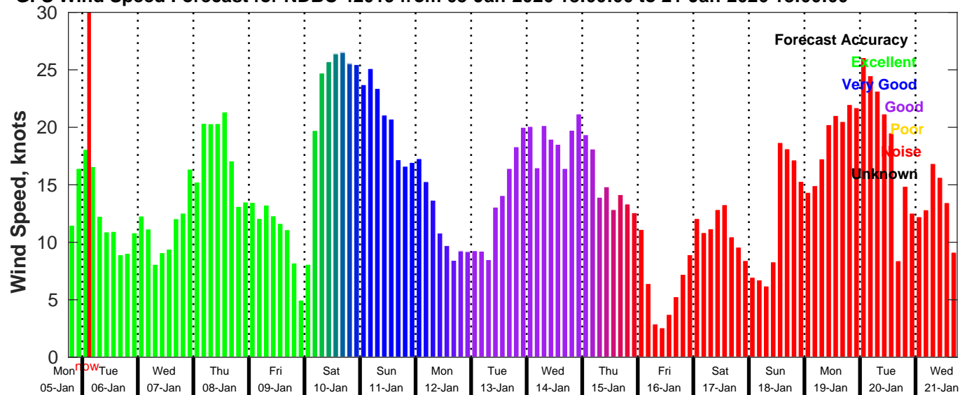
GFS Wind Speed Forecast for NDBC 42019 from 05-Jan-2026 18:00:00 to 21-Jan-2026 18:00:00
