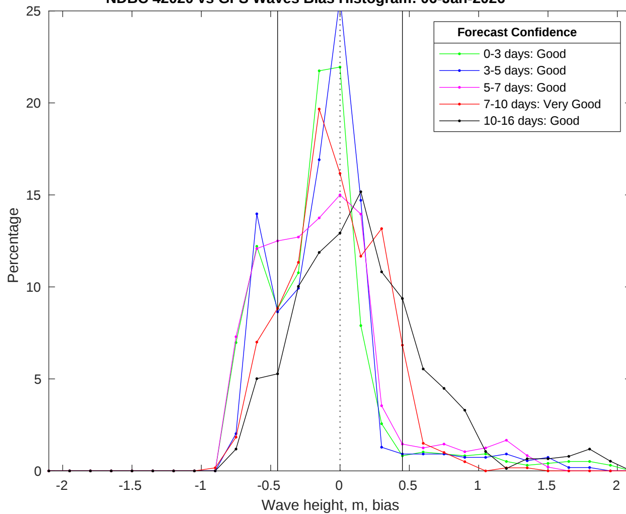
NDBC 42020 vs GFS Waves Bias Histogram: 06-Jan-2026
