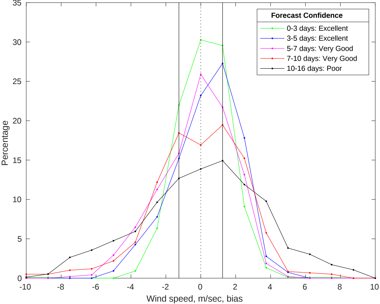
NDBC 42020 vs GFS Winds Bias Histogram: 06-Jan-2026
