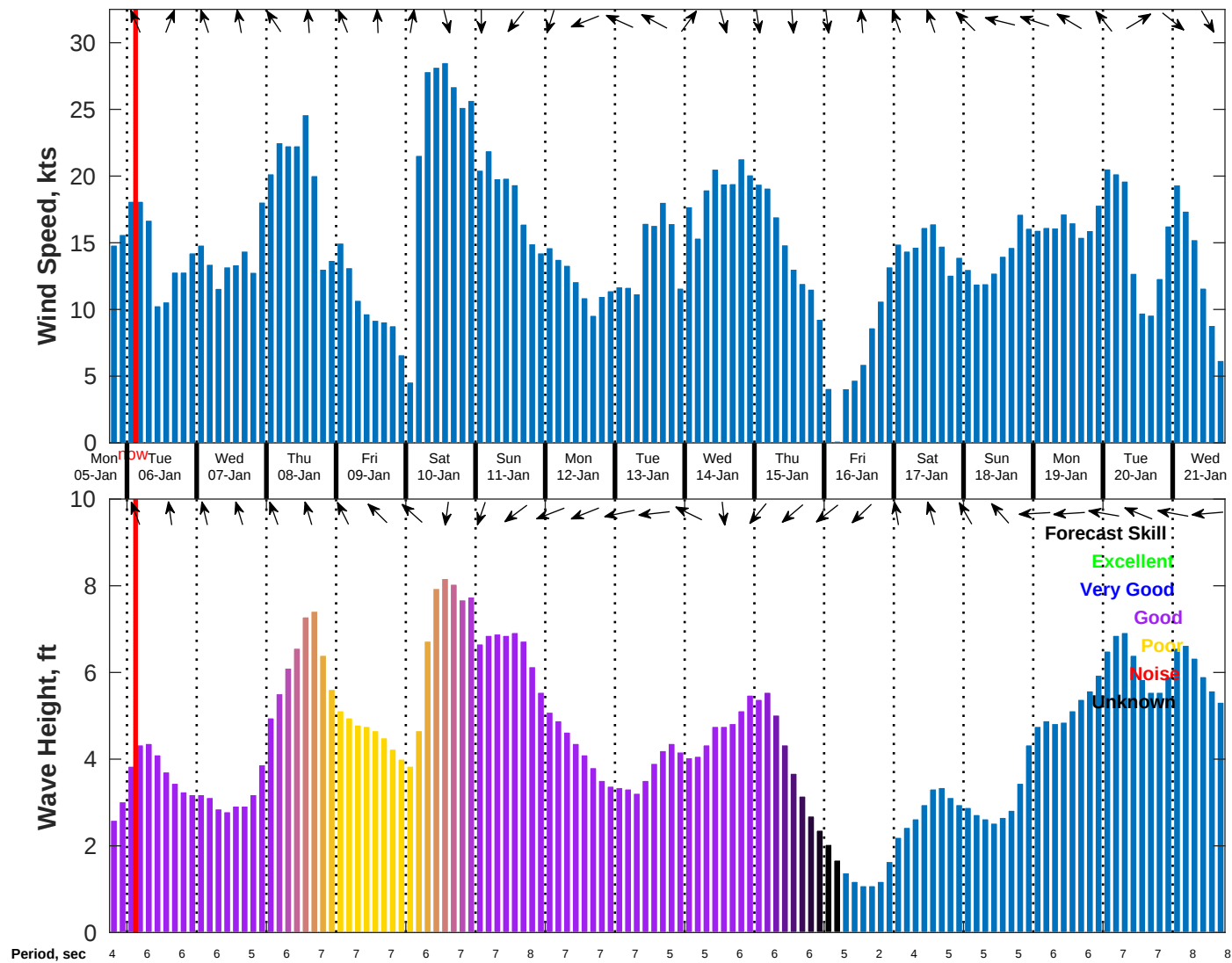
Wind & Wave Forecast for NDBC 42020 from 05-Jan-2026 18:00:00 to 21-Jan-2026 18:00:00
