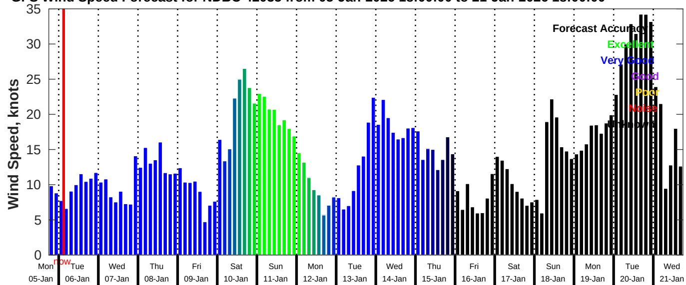
GFS Wind Speed Forecast for NDBC 42035 from 05-Jan-2026 18:00:00 to 21-Jan-2026 18:00:00
