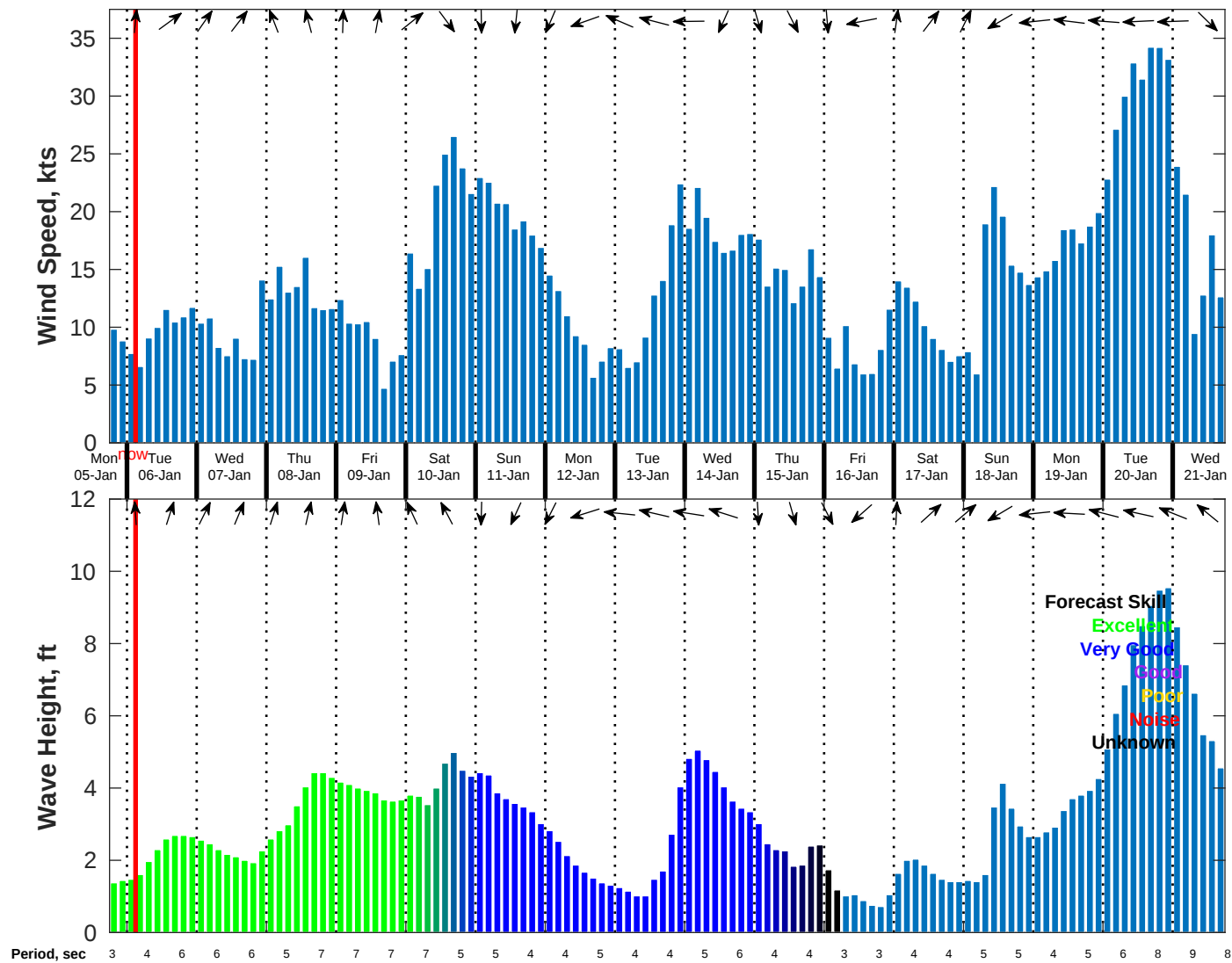
Wind & Wave Forecast for NDBC 42035 from 05-Jan-2026 18:00:00 to 21-Jan-2026 18:00:00
