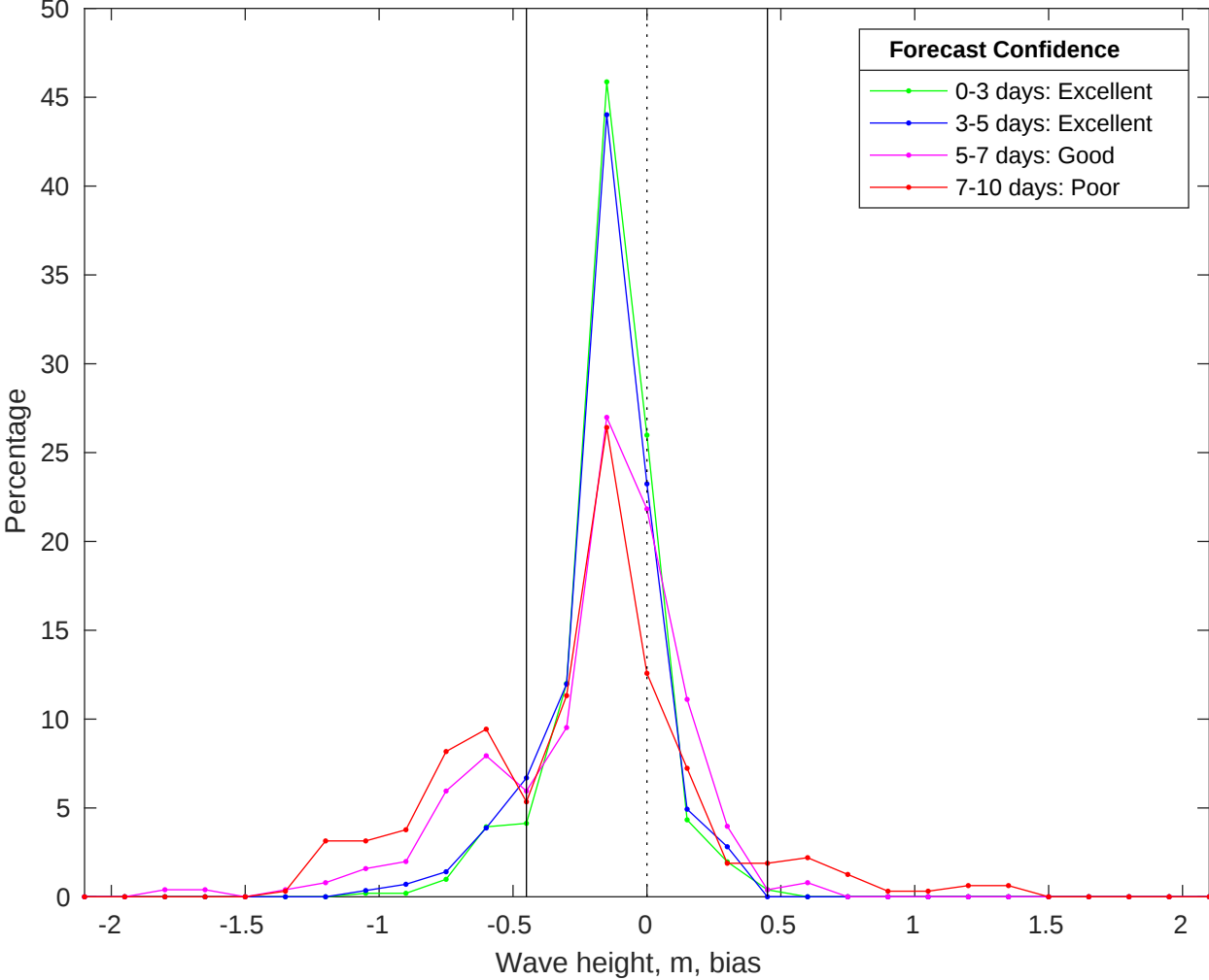
NDBC 42036 vs CMEMS Waves Bias Histogram: 06-Jan-2026
