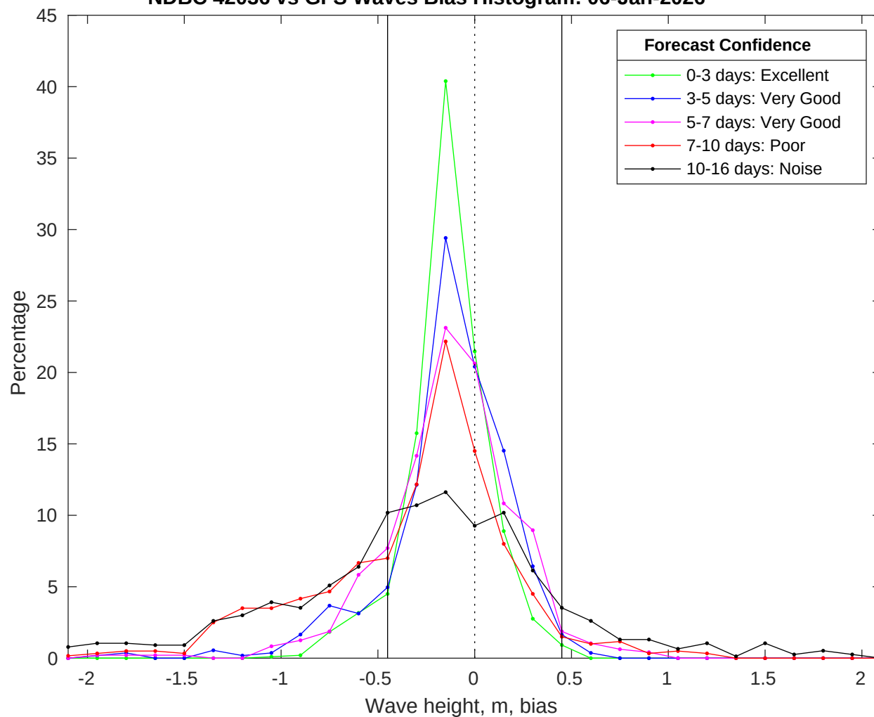
NDBC 42036 vs GFS Waves Bias Histogram: 06-Jan-2026
