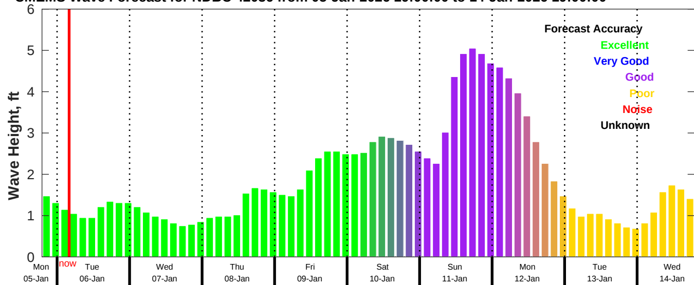
CMEMS Wave Forecast for NDBC 42036 from 05-Jan-2026 19:00:00 to 14-Jan-2026 19:00:00
