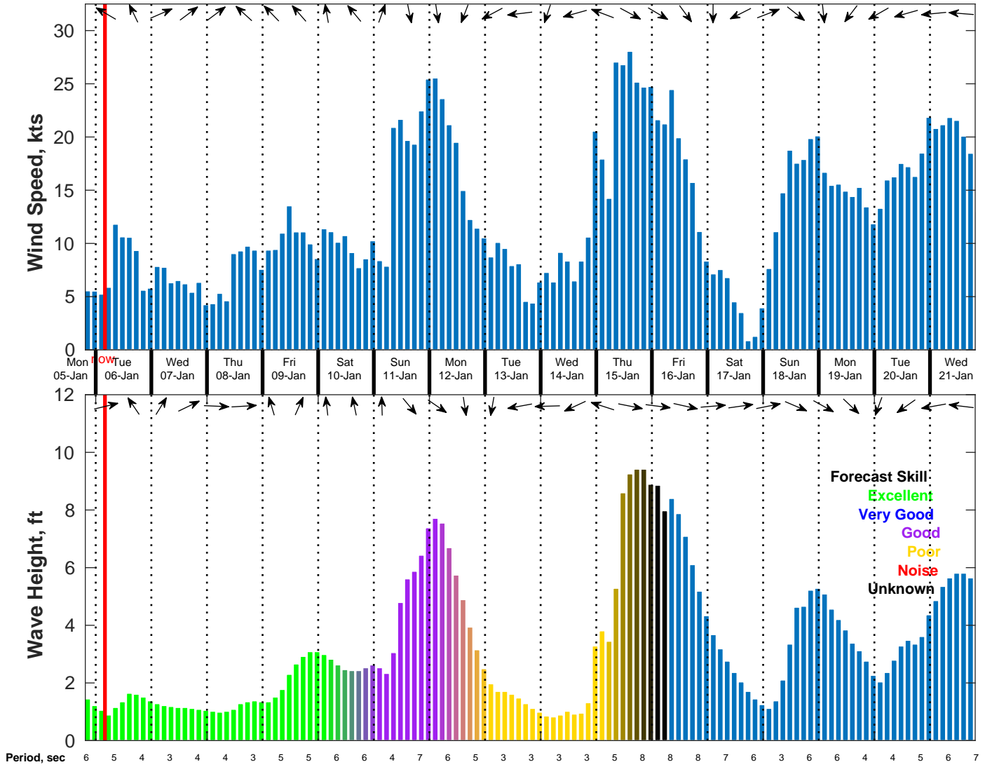
Wind & Wave Forecast for NDBC 42036 from 05-Jan-2026 19:00:00 to 21-Jan-2026 19:00:00
