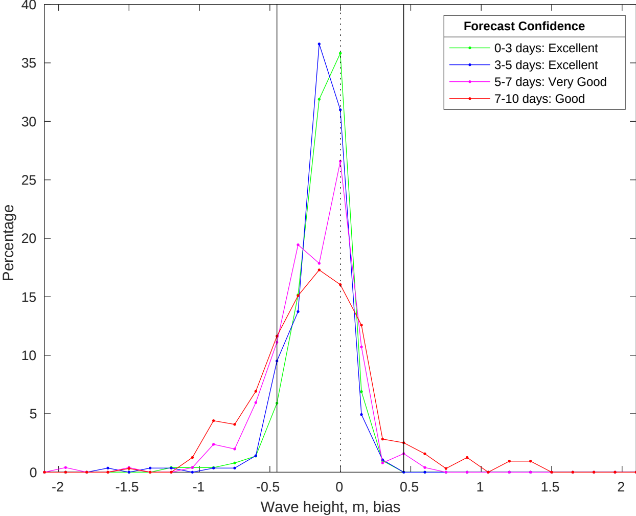
NDBC 42040 vs CMEMS Waves Bias Histogram: 06-Jan-2026
