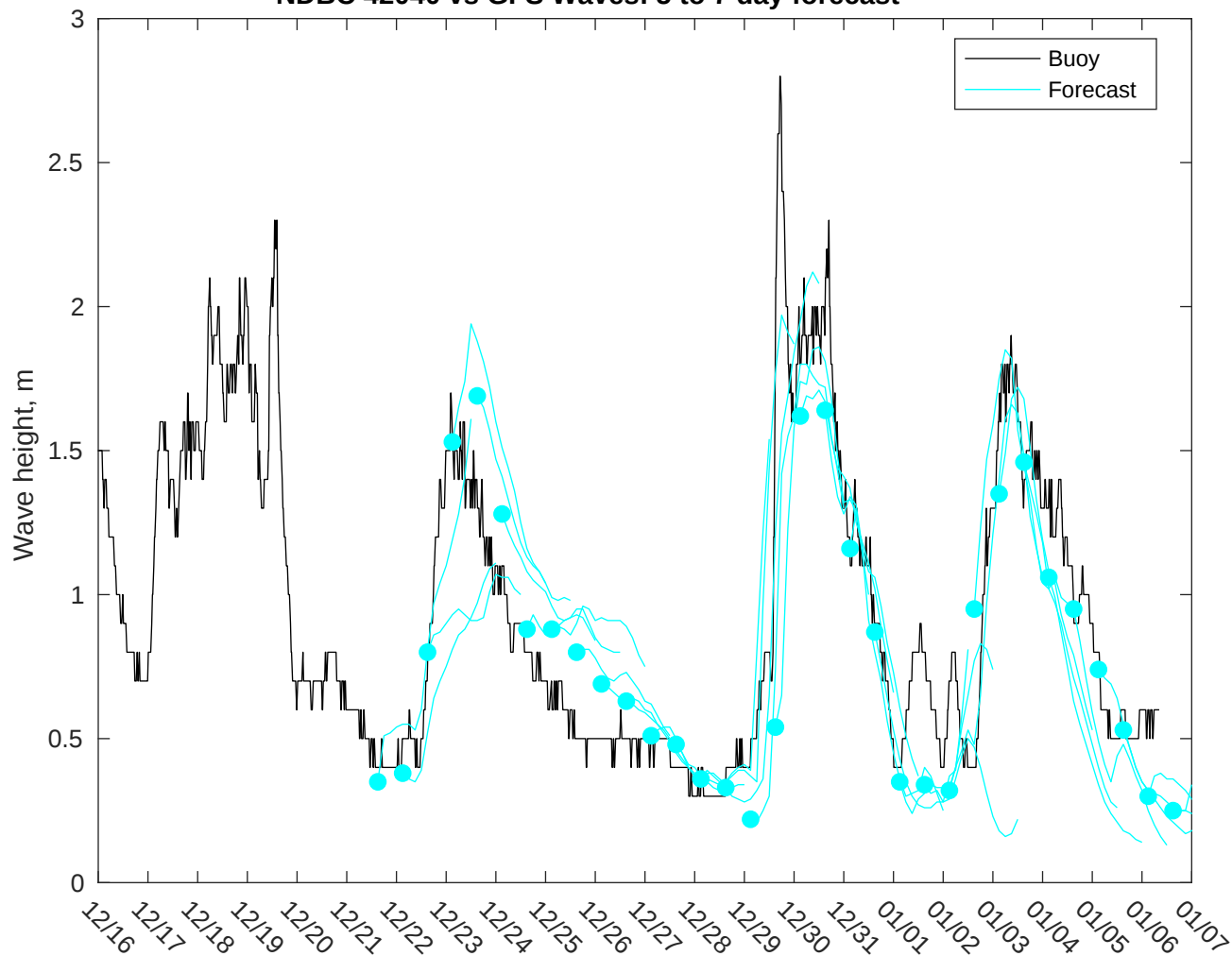
NDBC 42040 vs GFS Waves: 5 to 7 day forecast
