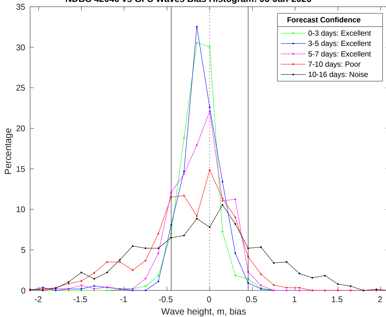
NDBC 42040 vs GFS Waves Bias Histogram: 06-Jan-2026
