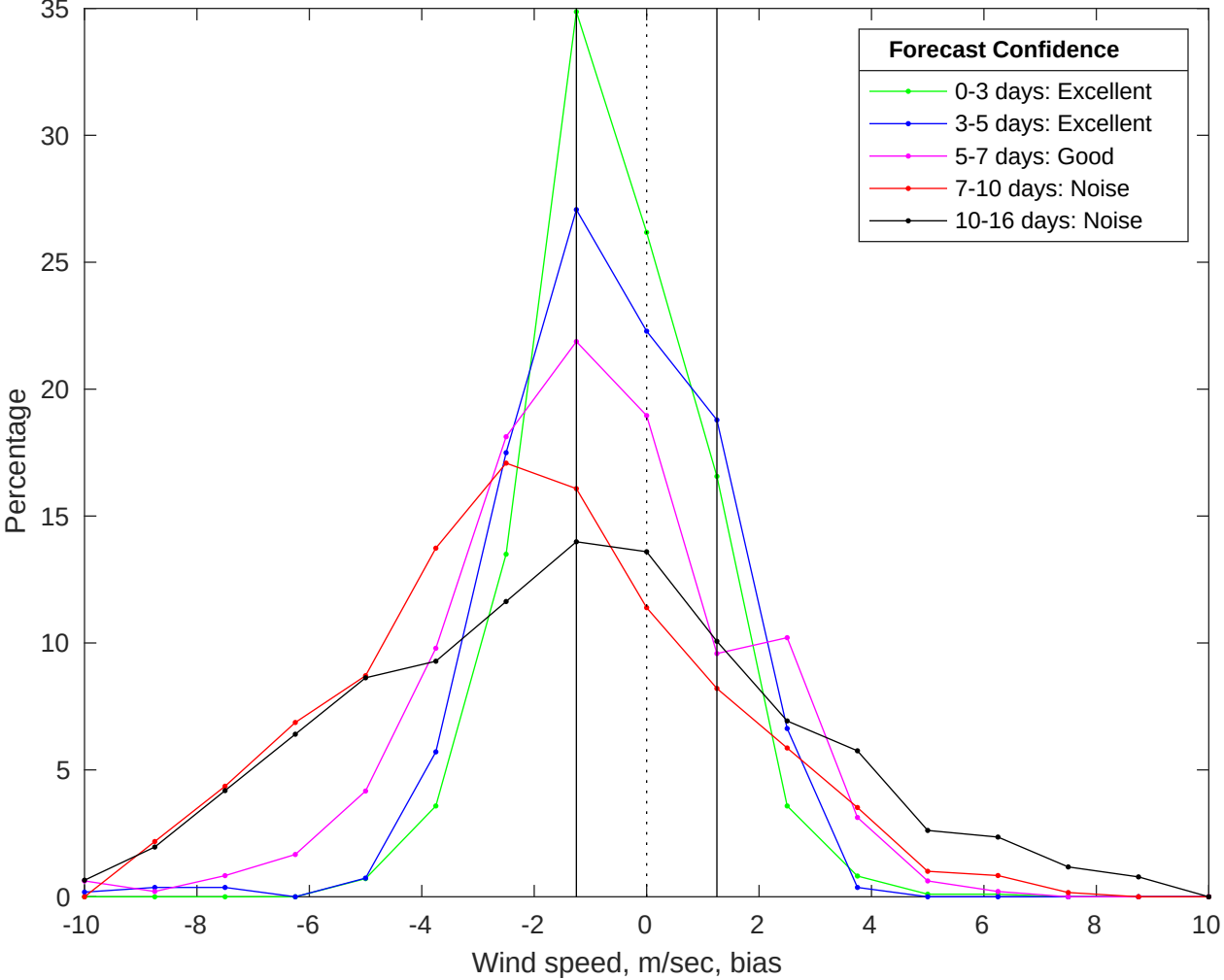
NDBC 42040 vs GFS Winds Bias Histogram: 06-Jan-2026
