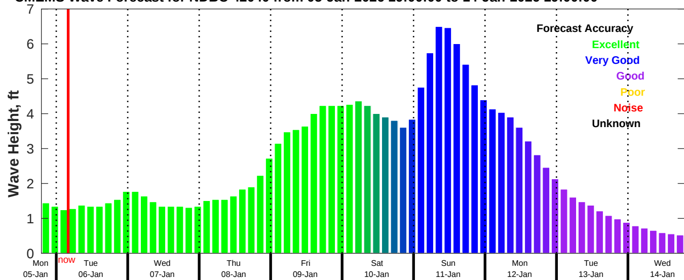
CMEMS Wave Forecast for NDBC 42040 from 05-Jan-2026 19:00:00 to 14-Jan-2026 19:00:00
