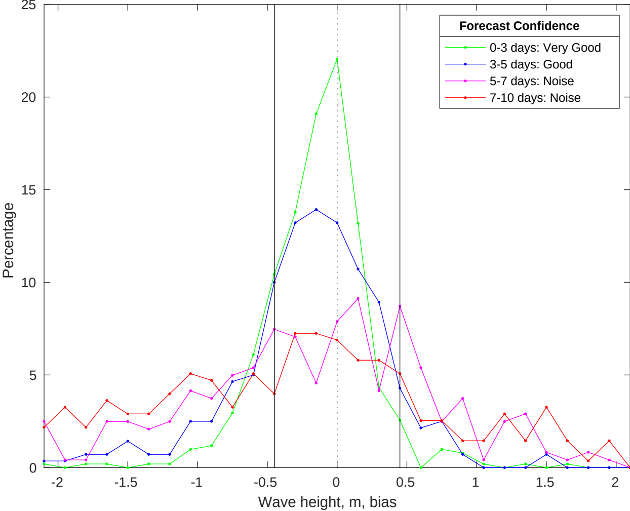
NDBC 44008 vs CMEMS Waves Bias Histogram: 06-Jan-2026
