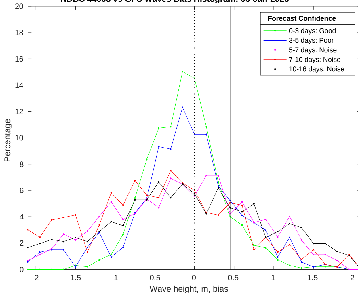
NDBC 44008 vs GFS Waves Bias Histogram: 06-Jan-2026
