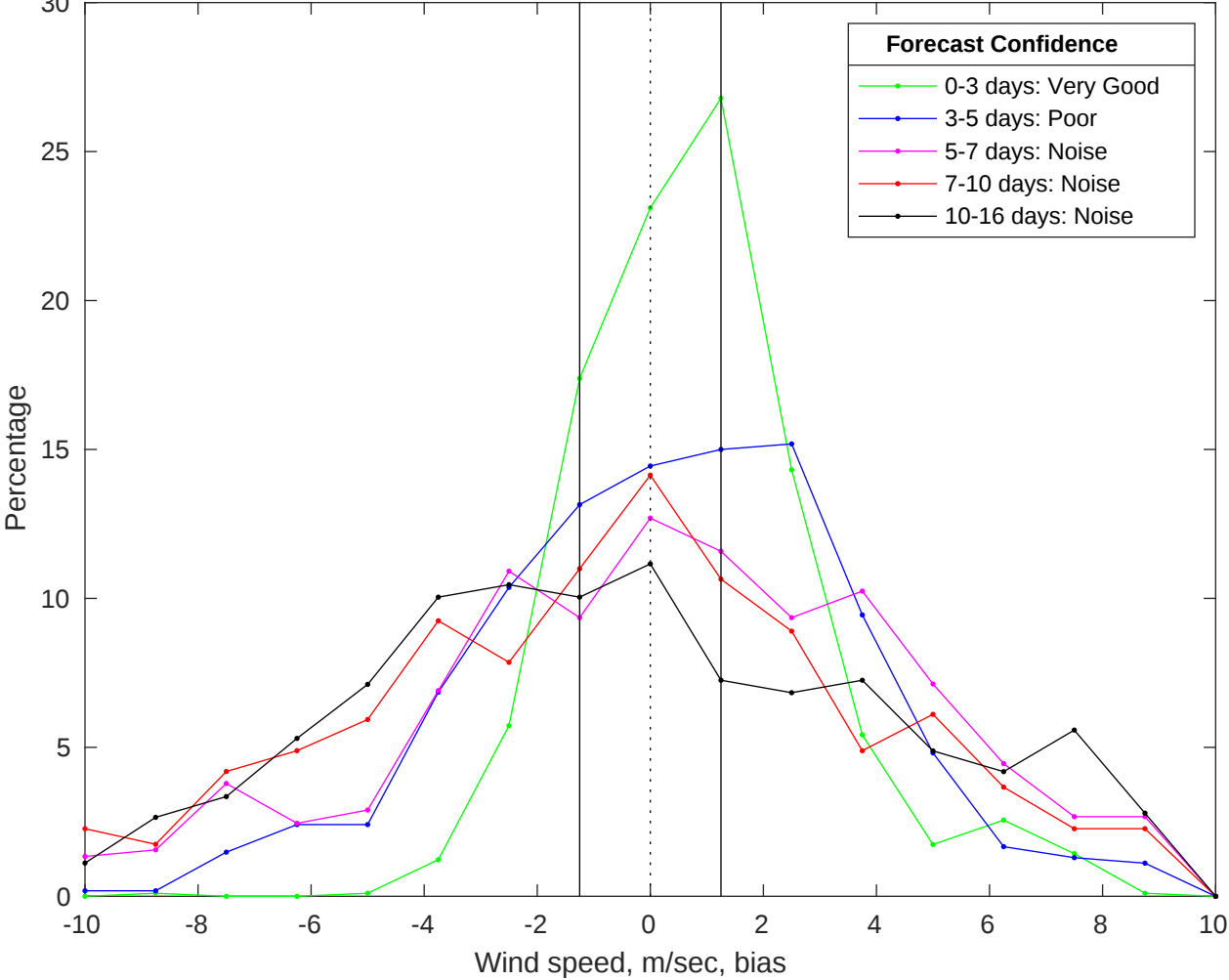
NDBC 44008 vs GFS Winds Bias Histogram: 06-Jan-2026
