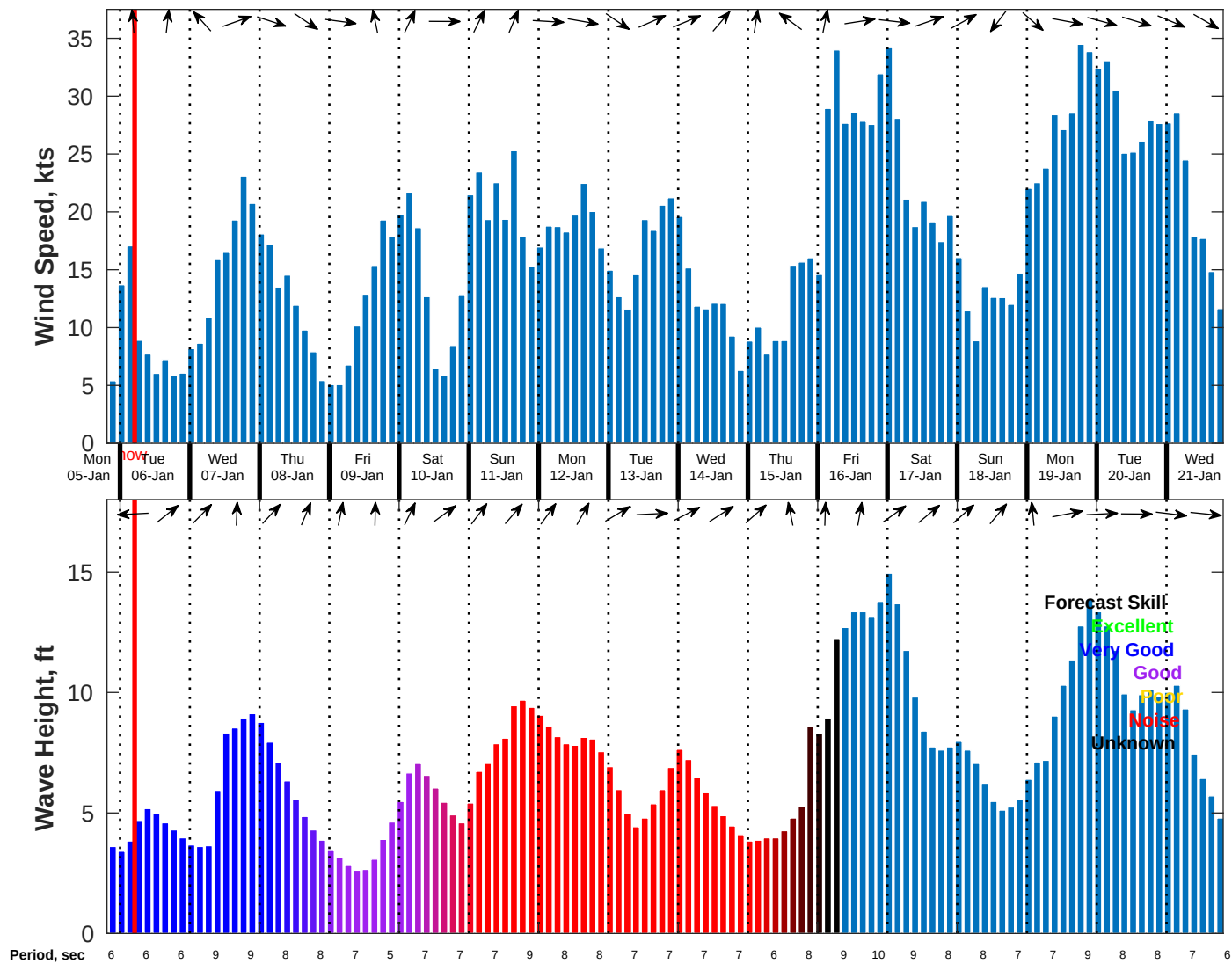
Wind & Wave Forecast for NDBC 44008 from 05-Jan-2026 20:00:00 to 21-Jan-2026 20:00:00
