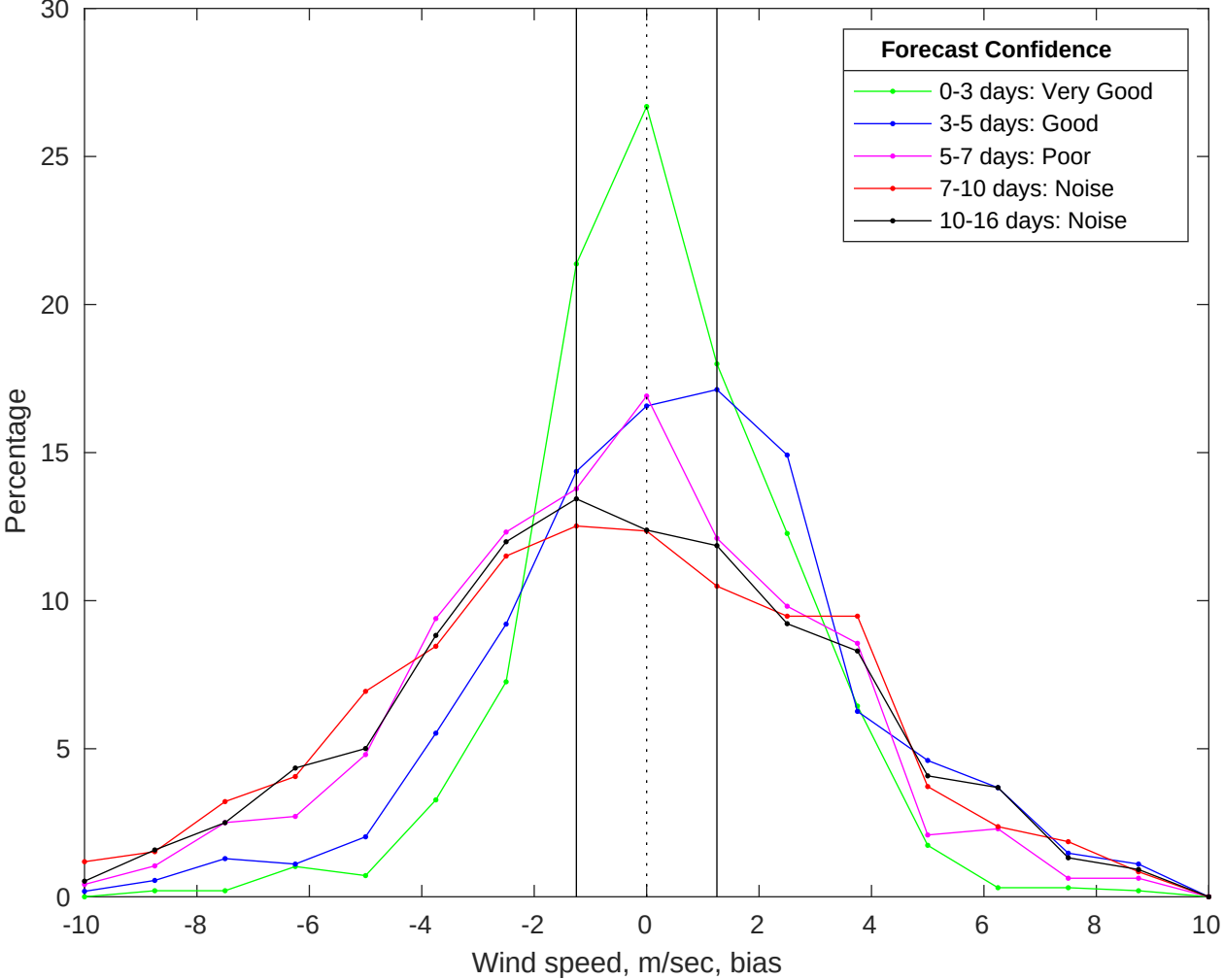
NDBC 46011 vs GFS Winds Bias Histogram: 06-Jan-2026
