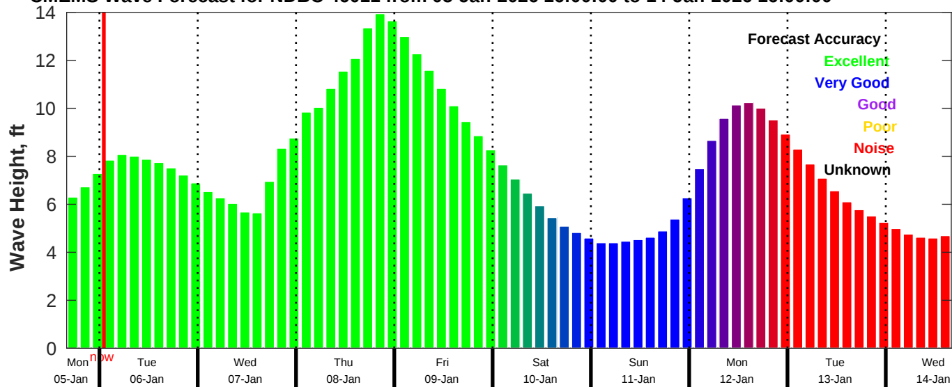
CMEMS Wave Forecast for NDBC 46011 from 05-Jan-2026 16:00:00 to 14-Jan-2026 16:00:00
