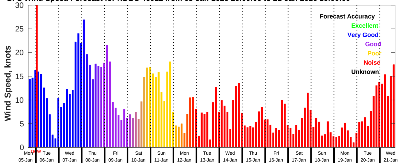
GFS Wind Speed Forecast for NDBC 46011 from 05-Jan-2026 16:00:00 to 21-Jan-2026 16:00:00
