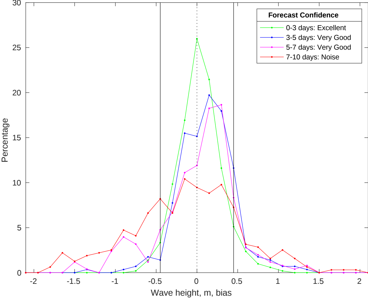
NDBC 46028 vs CMEMS Waves Bias Histogram: 06-Jan-2026
