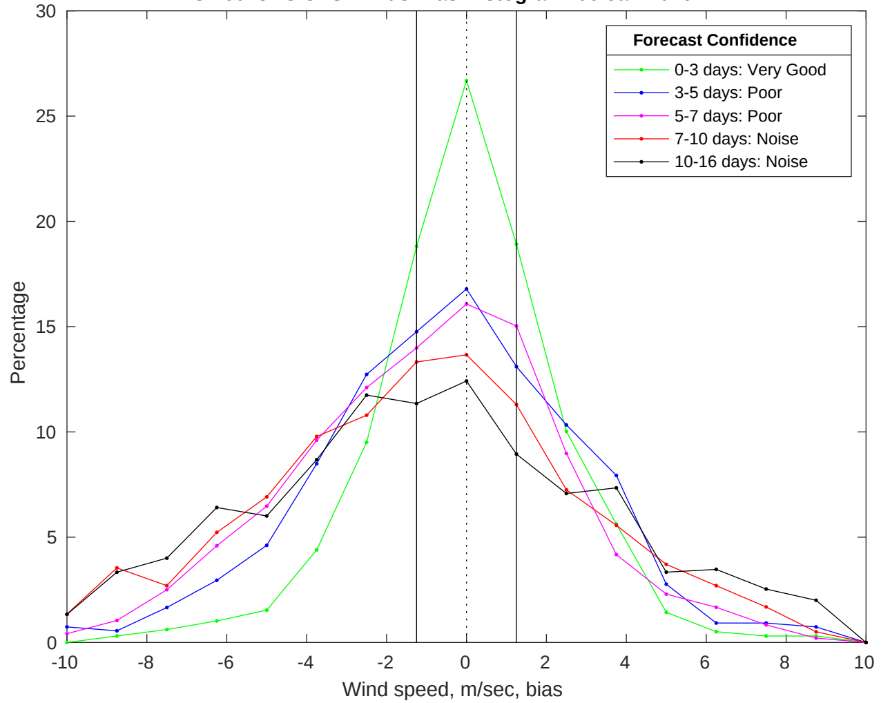
NDBC 46028 vs GFS Winds Bias Histogram: 06-Jan-2026
