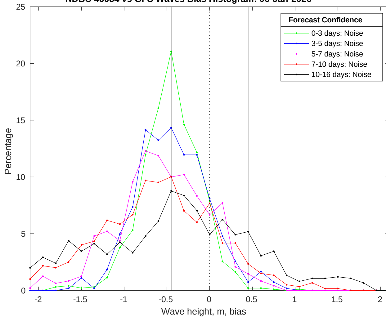
NDBC 46054 vs GFS Waves Bias Histogram: 06-Jan-2026
