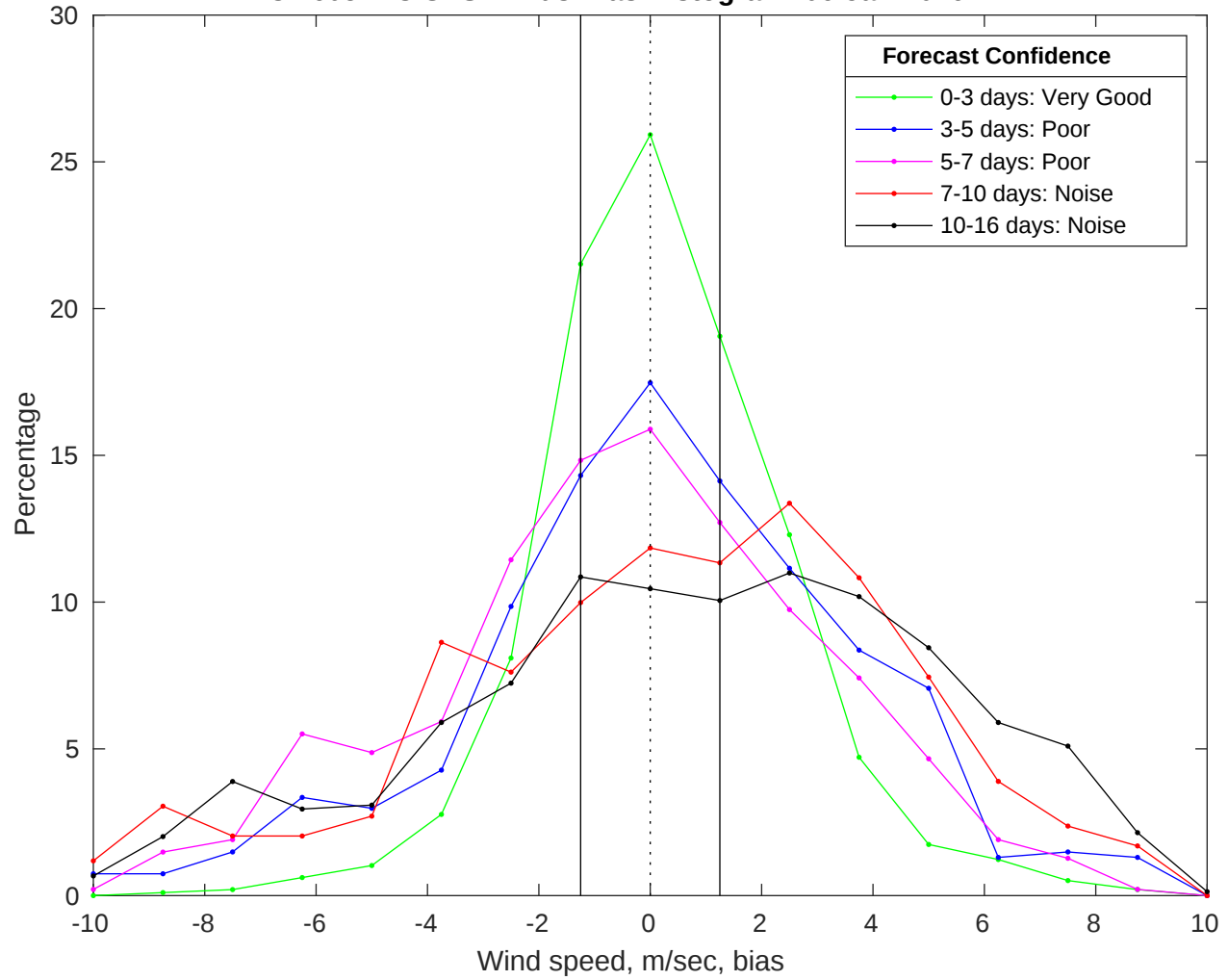
NDBC 46054 vs GFS Winds Bias Histogram: 06-Jan-2026
