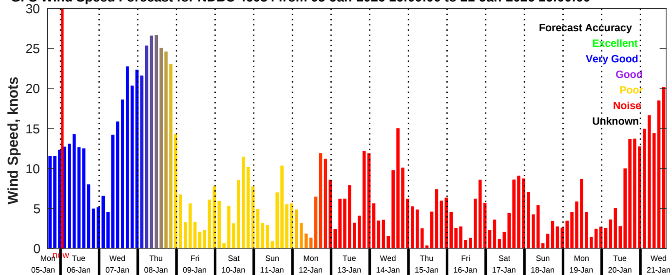
GFS Wind Speed Forecast for NDBC 46054 from 05-Jan-2026 16:00:00 to 21-Jan-2026 16:00:00
